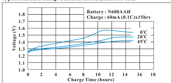
Typical Standard Charge Characteristics (Cylindrical Cell)
